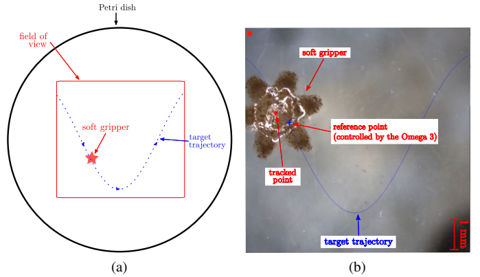
Fig. 6. Experiment #1: Path following task. Subjects are required to steer a soft gripper along the predetermined trajectory, being as fast and precise as possible. We considered four target trajectories and eight feedback conditions (a video is available as supplemental material).
