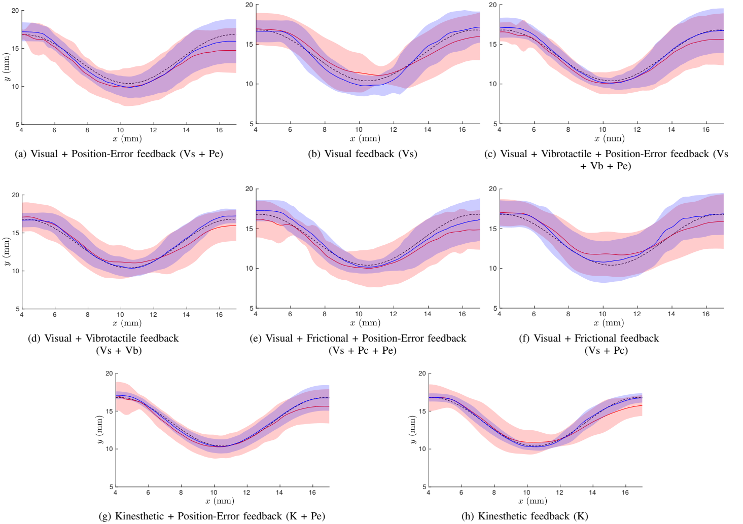
Fig. 7. Experiment #1: Path following task. Average trajectory of the reference point (blue) and the tracked gripper (red) along the x and y axes (solid lines) \pm standard deviation (patches) along the y axis is shown for each feedback condition for target trajectory 1 (black dashed line).
