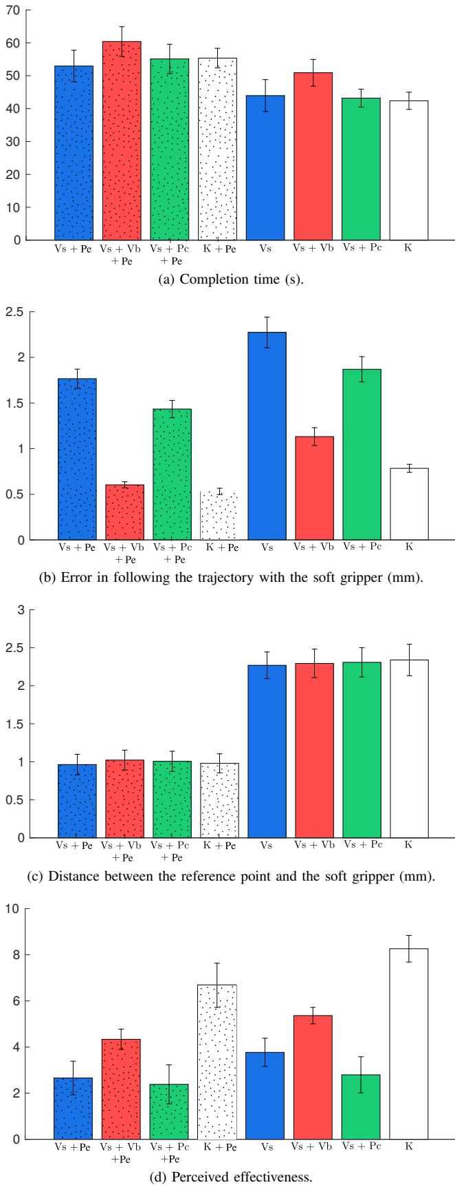
Fig. 8. Experiment #1: Path following task. Completion time, error in following the trajectory with the soft gripper, distance between the reference point and the soft gripper, and perceived effectiveness for the eight considered feedback conditions are plotted (mean and 95% confidence interval). A video of the experiment is available as supplemental material.
