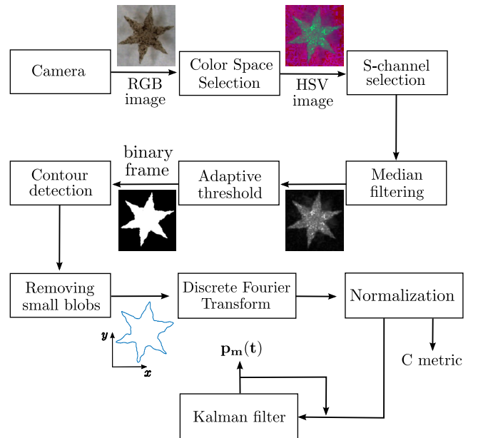
Fig. 3. Tracking algorithm. Each frame registered by the high-resolution camera is first converted to HSV colorspace, then its saturation channel (S) is filtered using a median filter, and a binary frame is obtained using an adaptive threshold. The binary frame is then used to find the contours of the image, and Fourier descriptors are used to detect the centroid of the microgripper and measure how much the microgripper has closed. Finally, a Kalman filter is used to deal with uncertainties in the tracking. The tracking system runs at 50 Hz.
