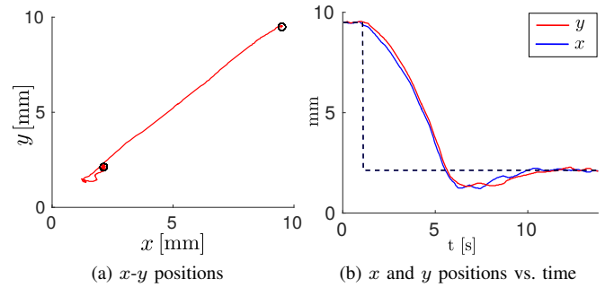
Fig. 5. Position control: A representative point-to-point positioning trial. The reference position of the gripper was suddenly changed and the trajectory of the gripper was registered. Solid lines show the position of the gripper in (a) space and (b) time. The commanded reference positions are shown as circles in (a) and as a dashed line in (b).
