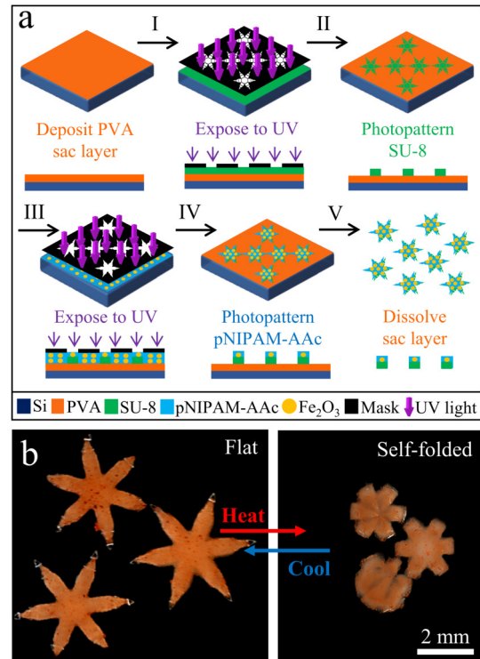
Fig. 2. Soft gripper fabrication and operation. (a) Schematic illustration of the process used to photopattern SU-8 and pNIPAM-AAc soft grippers. (b) Optical images showing the grippers closing on heating and opening up on cooling.
