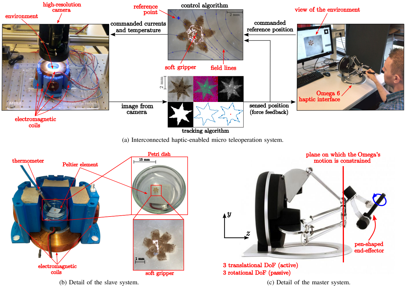
Fig. 1. Haptic-enabled micro teleoperation system. The image-guided algorithm tracks the position of the miniaturized soft gripper in the remote environment using a high-resolution camera and a Fourier-descriptors-based algorithm. A 6-DoF grounded haptic interface then provides the human operator with haptic stimuli about the interaction of the gripper with the remote environment. At the same time, it enables the operator to intuitively control the reference position of the gripper. Finally, the magnetic control algorithm steers the gripper toward the reference position defined by the operator, and a Peltier element regulates the temperature of the distilled water where the gripper is floating.
