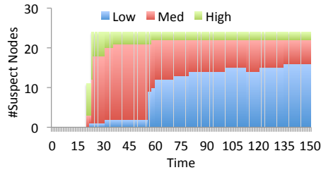
Fig. 12: Suspicion level changes over time
