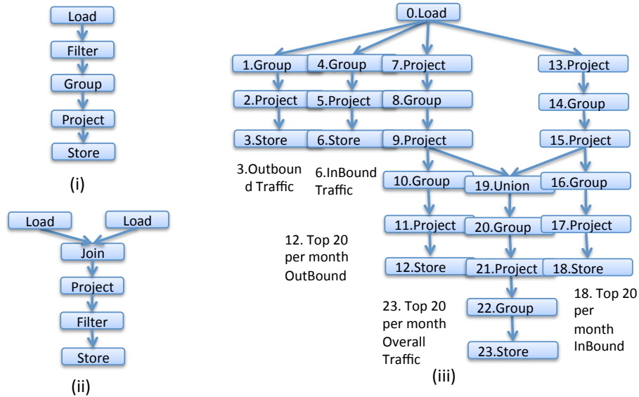
Fig. 8: Data-flow graph for (i) Twitter Follower Analysis (ii) Twitter Two Hop Analysis, (iii) Air Traffic Analysis
