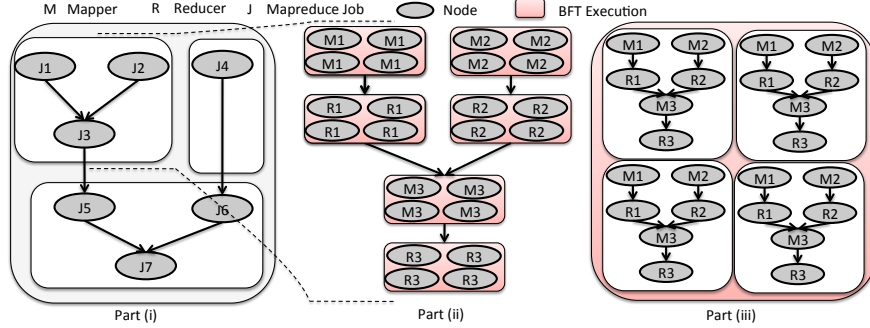
Fig. 1: Part (i) shows a data-flow graph with 7 phases. (ii) focuses on n \times m replication of jobs J1, J2 and J3. (iii) shows clustered replication of J1, J2, J3 requiring only one round of BFT consensus. For simplicity we only show one map and one reduce task per MapReduce job.
