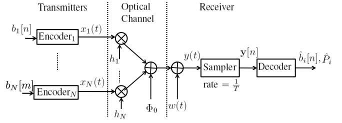
Fig. 1: A channel model of an VLC system for broadcasting N data streams by N transmitters which are asynchronous.
