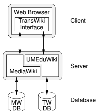
Fig. 1. TransWiki system structure
