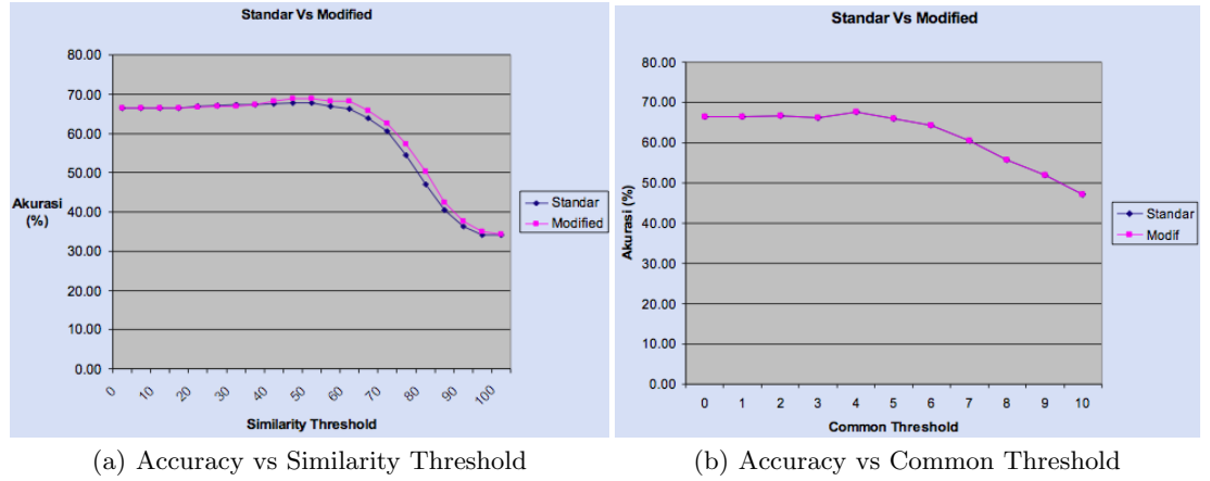
Fig. 2. Accuration versus Similarity Threshold or Common Threshold
