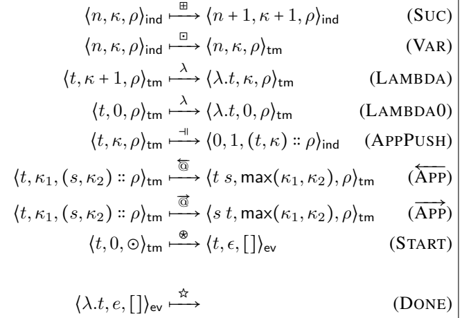
Fig. 7: Contextual equivalence machine
