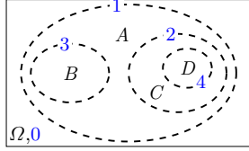
(c) The level lines of \omega_{TV}
