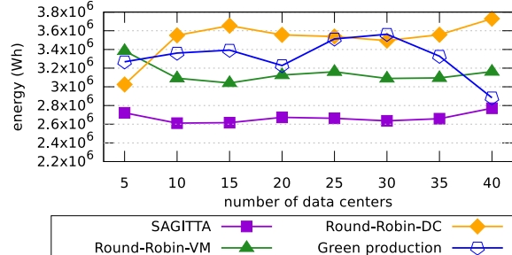
Figure 10: Brown energy consumption of SAGITTA with increasing number of data centers.
