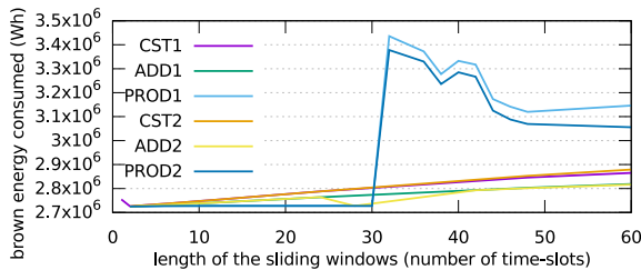
Figure 8: Influence of Eg_i estimation.
