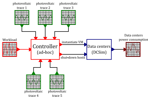
Figure 2: Bloc diagram view of the cloud model.
