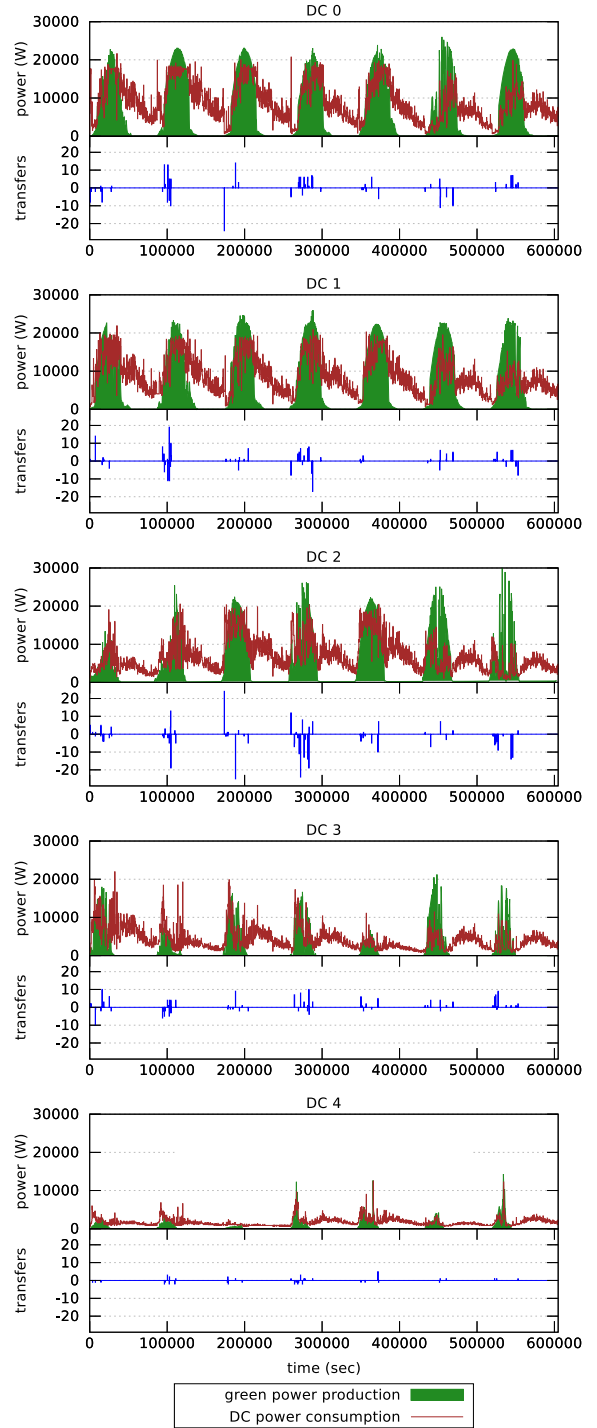
Figure 6: Power consumption per data center with SAGITTA and transfer decisions.
