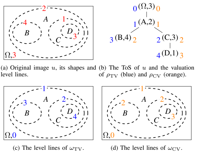
Fig. 7. Equivalence between the level lines of a gray-level image u and the level lines of the distance maps \omega_{TV} and \omega_{CV} .
