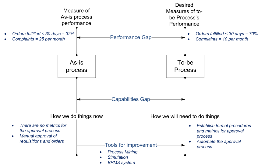
Fig. 5. Gap analysis
