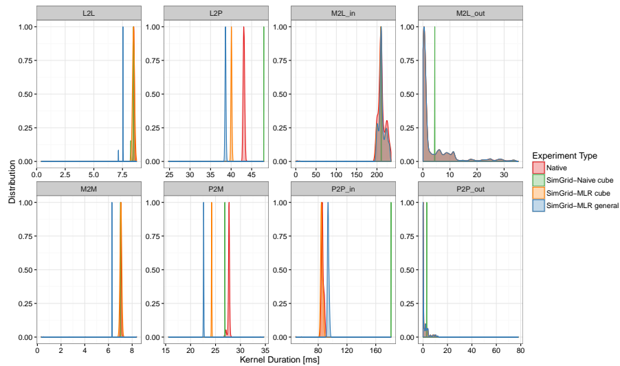
Figure 10: Kernel duration distributions. For many kernels, MLR models are completely overlapped with the Native distribution.
