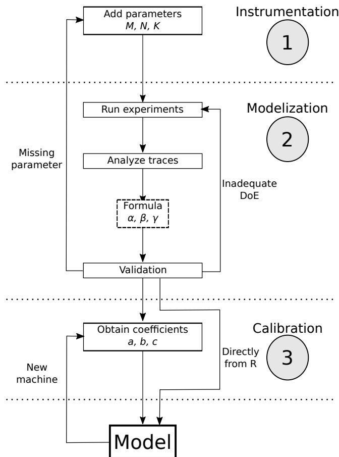
Figure 4: Summary of the kernel modeling workflow. The process is divided into three phases and although it is essentially linear, several loopbacks are often needed due to the missing parameters or initially inadequate design of experiments.
