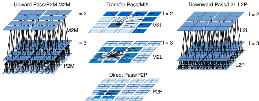
Figure 2: Different steps of the FMM algorithm; upward pass (left), transfer pass and direct step (center), and downward pass (right).
