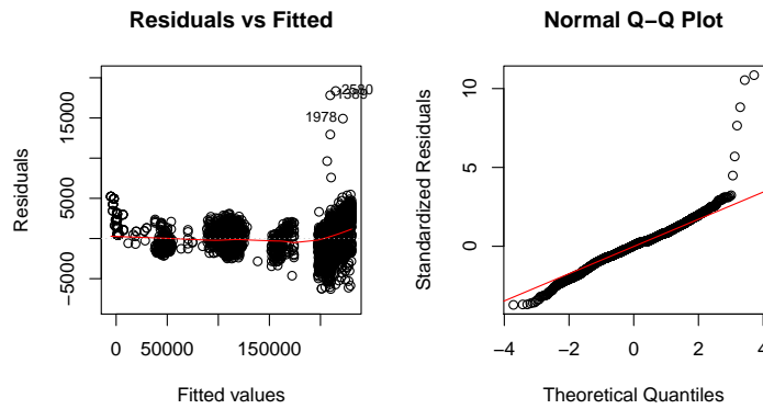
Figure 6: M2L.in model analysis when additional parameter (number of interactions) is added. Simpler model, higher adjusted R^2 , smaller and unstructured residuals and a normal distribution all suggest that this model is much more accurate than the initial one in Figure5
