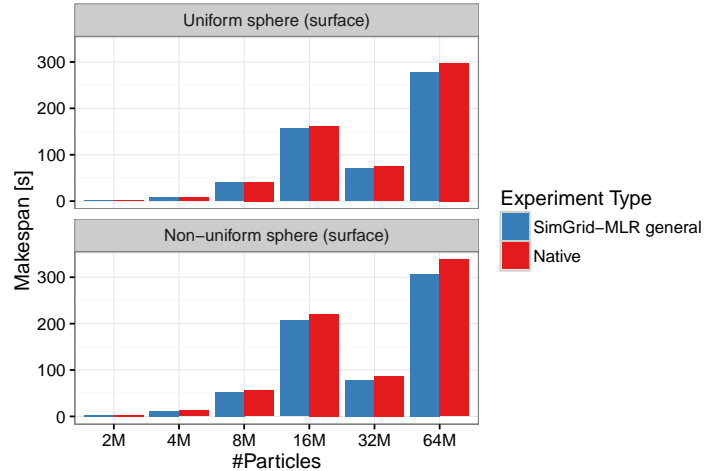
Figure 11: Simulation predictions for the uniform and non-uniform sphere use cases with different configuration options (particles, level and granularity).
