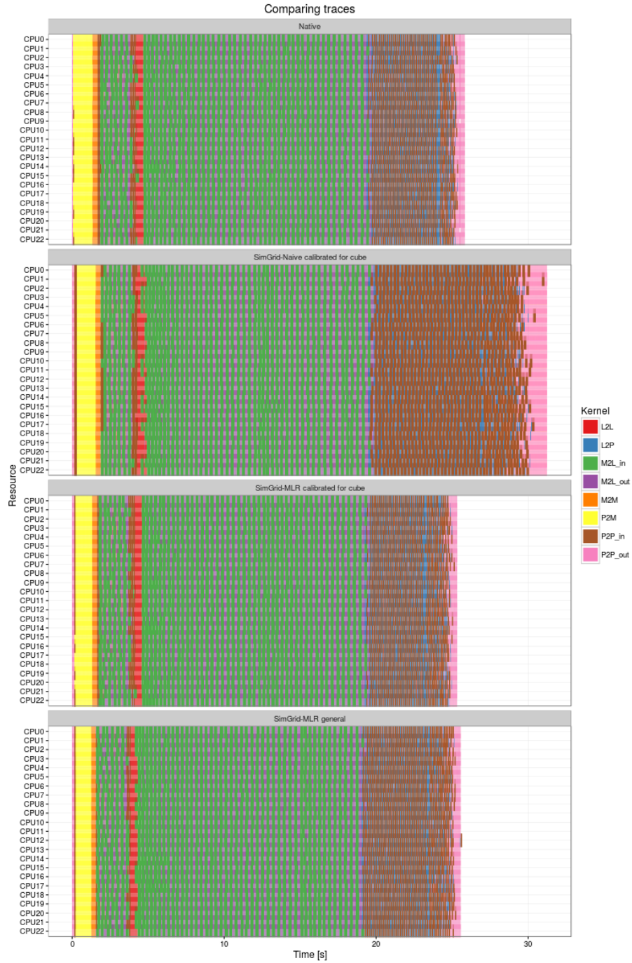
Figure 8: Even if runtime scheduler is dynamic, execution traces of Native and SimGrid-MLR match almost perfectly, while SimGrid-Naive execution is much longer.
