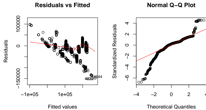
Figure 5: Initial model for M2L.in kernel. All parameter combinations (except IntervalSize 2 ) appear to be important, which is often a sign of overfitting. The residuals are structured and the distribution on Q – Q plot is skewed, which both suggest a missing parameter.
