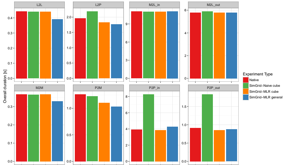
Figure 9: Comparing overall duration for each computation kernel between Native and SimGrid executions. The values are divided by the total number of CPU cores (23) to ease the comparison to the Figure8 and allow better estimation of the overall influence of each kernel.
