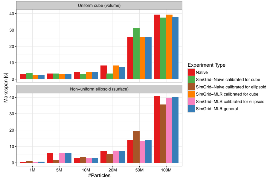
Figure 7: Overall execution time measured on a real machine (Native) and predicted by simulation (SimGrid). Simulation predictions with MLR models are very accurate, regardless of the particle distribution, number of particles, tree level or granularity.
