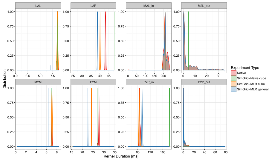
Figure 10: Kernel duration distributions. For many kernels, MLR models are completely overlapped with the Native distribution.
