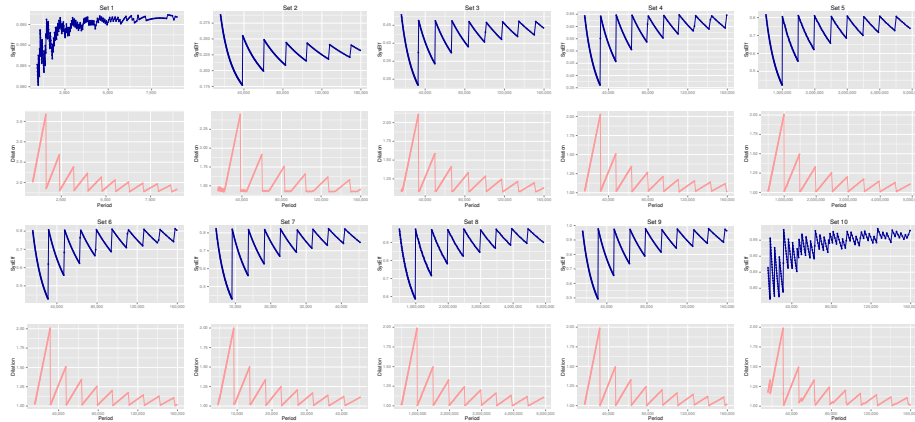
Figure 6: Evolution of SYSEFFICIENCY and DILATION when the pattern size increases.
