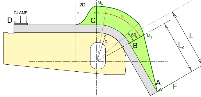
Fig. 3. Kinematics and moment distribution used as basis for development of steering model.
