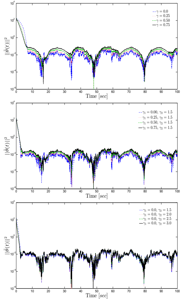
Figure 4. Parameter Identification Error Disturbance-Case. The top graph shows the parameter identification error for different values of \gamma \in (0, 1) (algorithm (4)), the bottom graph for the case \gamma_1 = 0 and \gamma_2 \in [1.5, 3.0] , while the middle graph for the case \gamma_1 \in (0, 1) and \gamma_2 = 1.5 (algorithm (8)), with \theta(0) = (0, 1)^T and \hat{\theta}(0) = (10, 10)^T .
