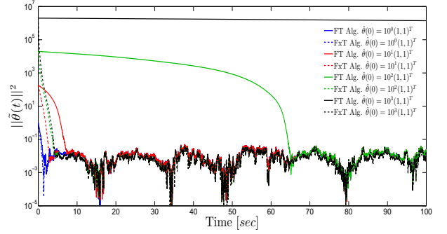
Figure 3. Parameter Identification Error - Disturbance Case
