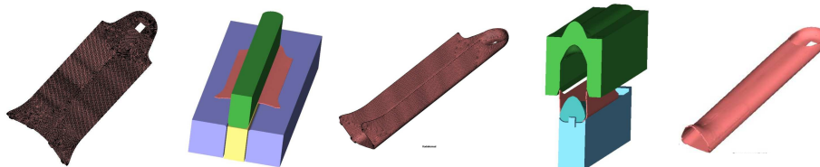
Fig. 6. Numerical models for FE analysis of virtual manufacturing
