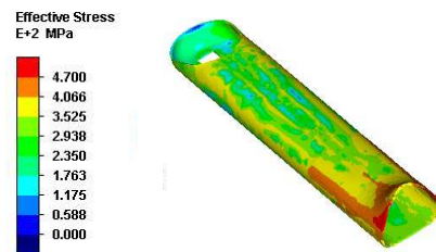
Fig. 8. Effective stress - 2 nd stage
