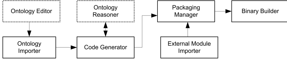
Fig. 2. Framework Methodology Software Realization Architectural Components
