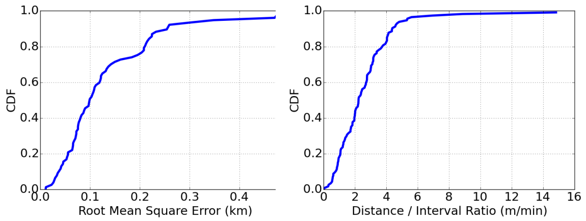
Figure 11: Distribution of the RMSE incurred by Figure 10. Distribution of the ratio between the average Haversine distance and the sampling interval as linear for all users.
