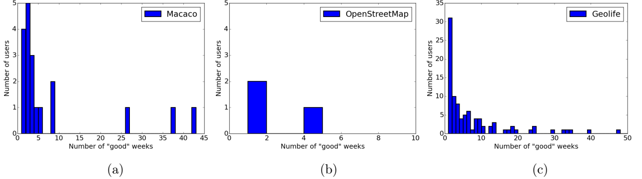
Figure 4: Distribution of one-week trajectories in our reference dataset, separated by data source. (a) MACACO. (b) OpenStreetMap. (c) GeoLife.
