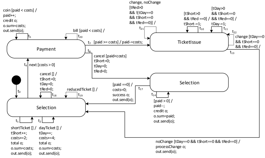
Fig. 8. Product Example: State Machine Model of a Ticket Machine without Bills, Change, and ReducedFare.
