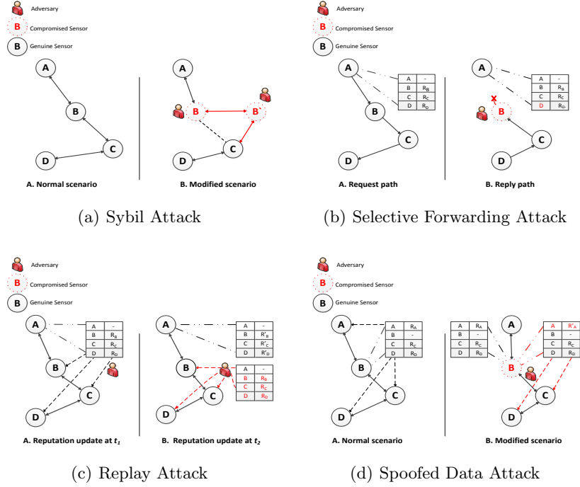
Fig. 1. Wireless sensor networks attacks: (a) Sybil Attack, (b) Selective Forwarding Attack, (c) Replay Attack, (d) Spoofed Data Attack .
