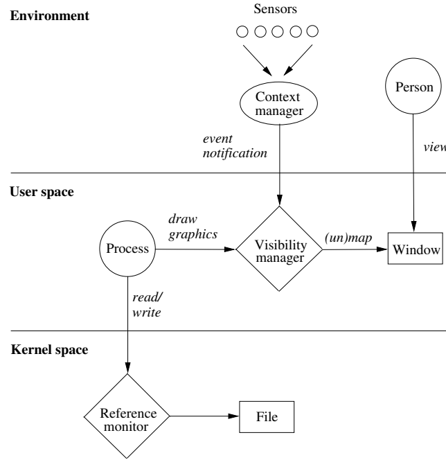
Fig. 2. Our adaption of the SEAC model to the Unix platform.
