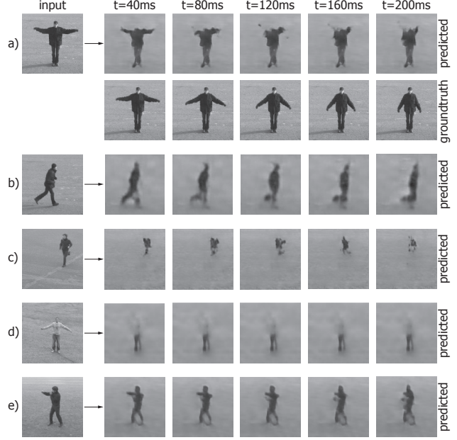
Figure 6. Examples of poor performing future anticipations: a) loss of details in waving, b) loss of details in jogging, c) extreme loss of details in running, d) loss of details with low contrast and e) artifacts in boxing.
