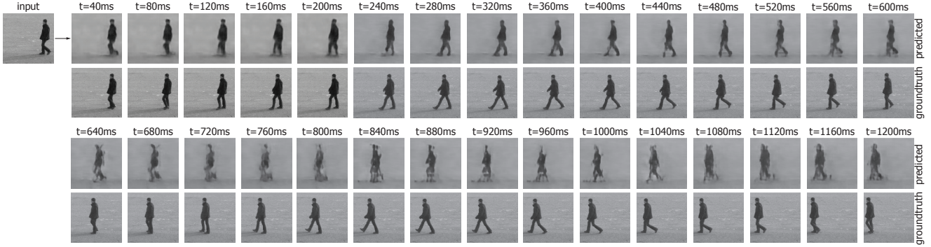
Figure 3. Long distance predictions. For larger temporal displacements artifacting becomes visible. The anticipated location of the person begins to differ from the groundtruth for even larger temporal differences, towards the end of the total motion duration.
