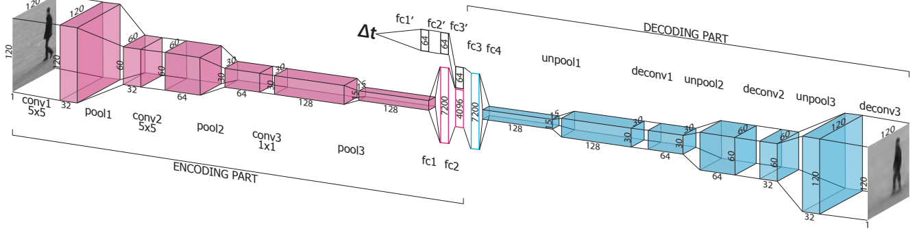
Figure 1. Our proposed architecture consists of two parts: i) an encoder part consisting of two branches: the first one taking the current image and the second one taking an arbitrary time difference t to the desired prediction and ii) a decoder part that generates an image, as anticipated, at the desired input time difference.
