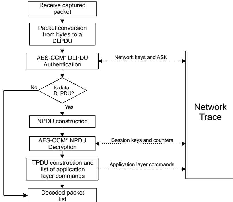
Fig. 5. Packet decoding sequence
