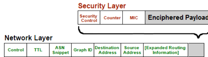
Fig. 2. NPDU structure
