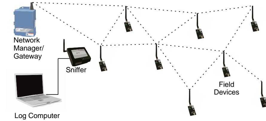
Fig. 7. Deployed network representation
