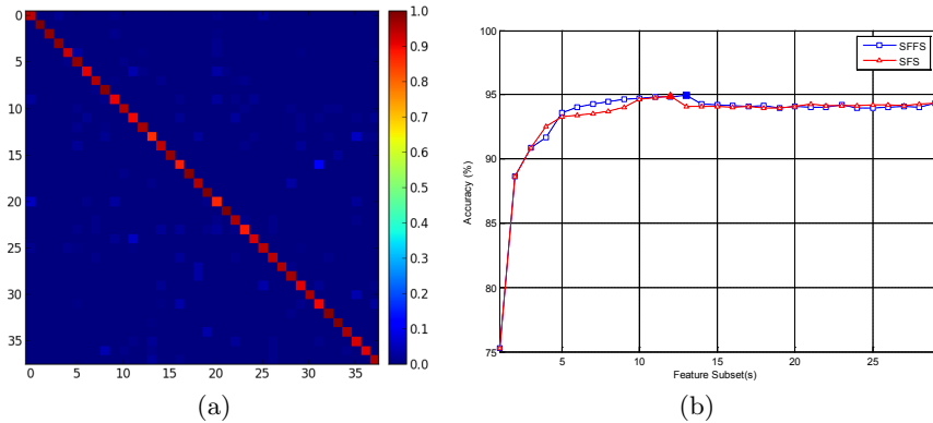
Fig. 6. (a) Confusion matrix of the gait recognition using SVM and RBF kernel with C = 2^{3.5} , = 2^{-5.25} , (b) the classification accuracy of various amounts of feature subsets by applying SFSS and SFS algorithm
