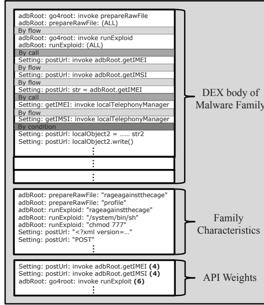
Signature example of malware family DroidDream
