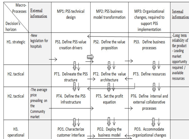
GRAI grid Ecobel "reference model"
