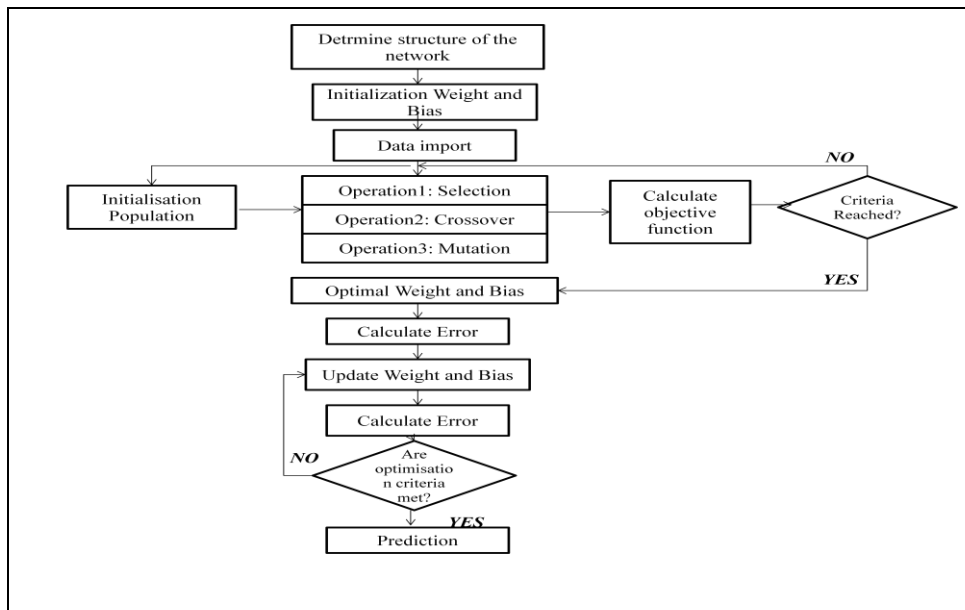
Fig. 1. The flow chart of RO-NN based on GA in the learning step. The algorithm is formed by three steps:
