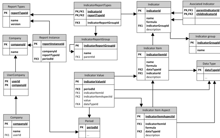
Fig. 2. Core data model of the reporting system
