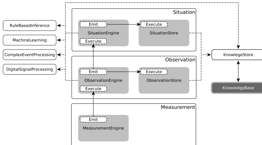
Fig. 1. System architecture for the representation of situational knowledge acquired from sensor measurement data showing the three layers of measurement, observation, and situation as well as the main components and modules, and their interactions.
