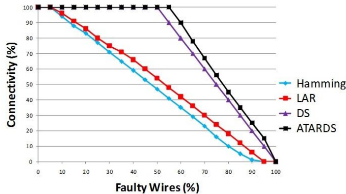
Fig. 6. NoC connectivity percentage in a generic 12-core NoC with MPEG4 benchmark.
