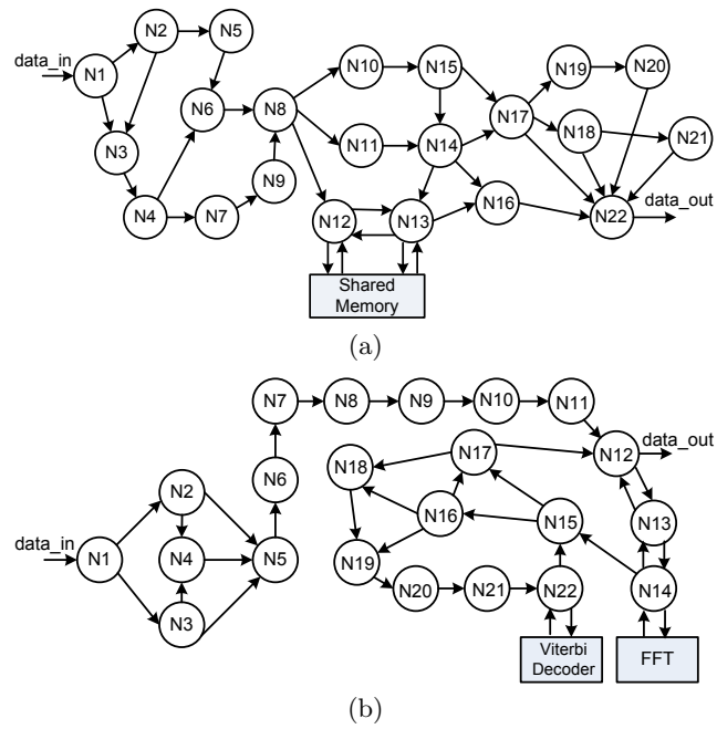
Fig. 8. Task graph of (a) a 22-node H.264/AVC video residual encoder, and (b) a 22-node 802.11a WLAN baseband receiver.
