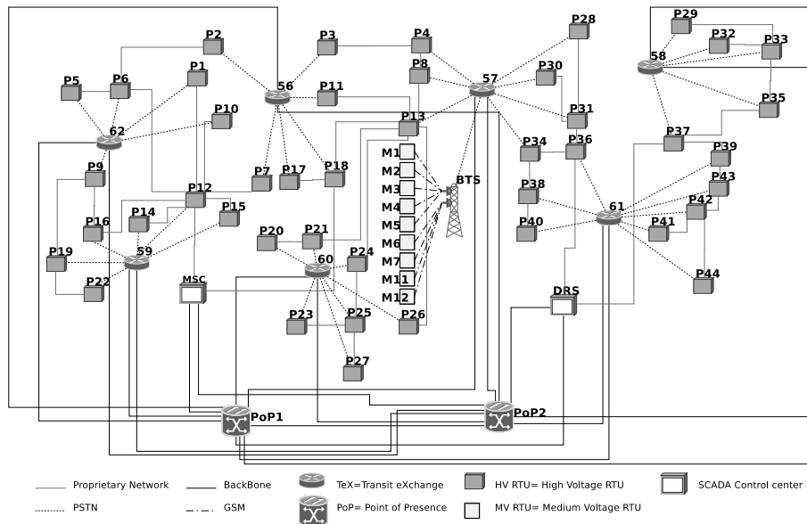
Figure 3. SCADA system.
