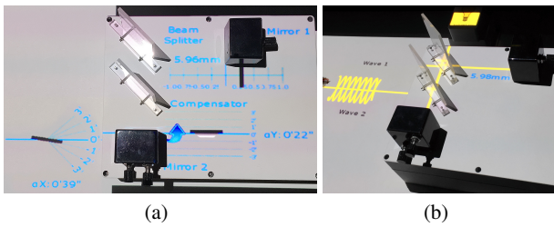
Figure 6. (a) Augmented information displayed next to the mirrors. The blue arrow indicates that Mirror 2 is being tilted forward, and the current angle is 0'22". The drawing on the left gives an indication of the x orientation of Mirror 2, and the graduated linear scale on top magnifies the current position of Mirror 1. (b) Light path and waves combination.
