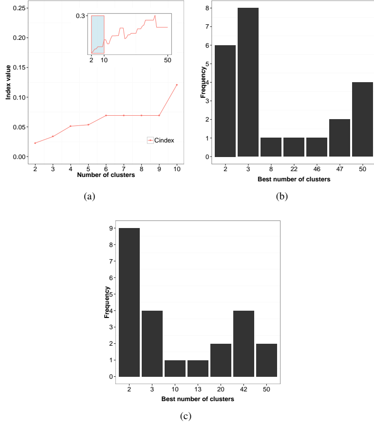
Figure 6: (a) C-Index values and respective number of clusters when re-clustering subscribers at the 3rd defined “traffic-volume”-based cluster, according to the number of sessions similarity. (b) Histogram of best number of “traffic-volume”-based clusters indicated by the assessed stopping rules. (c) Histogram of the best number of “number of sessions”-based clusters indicated, when re-clustering subscribers using the second “traffic-volume”-based cluster.
