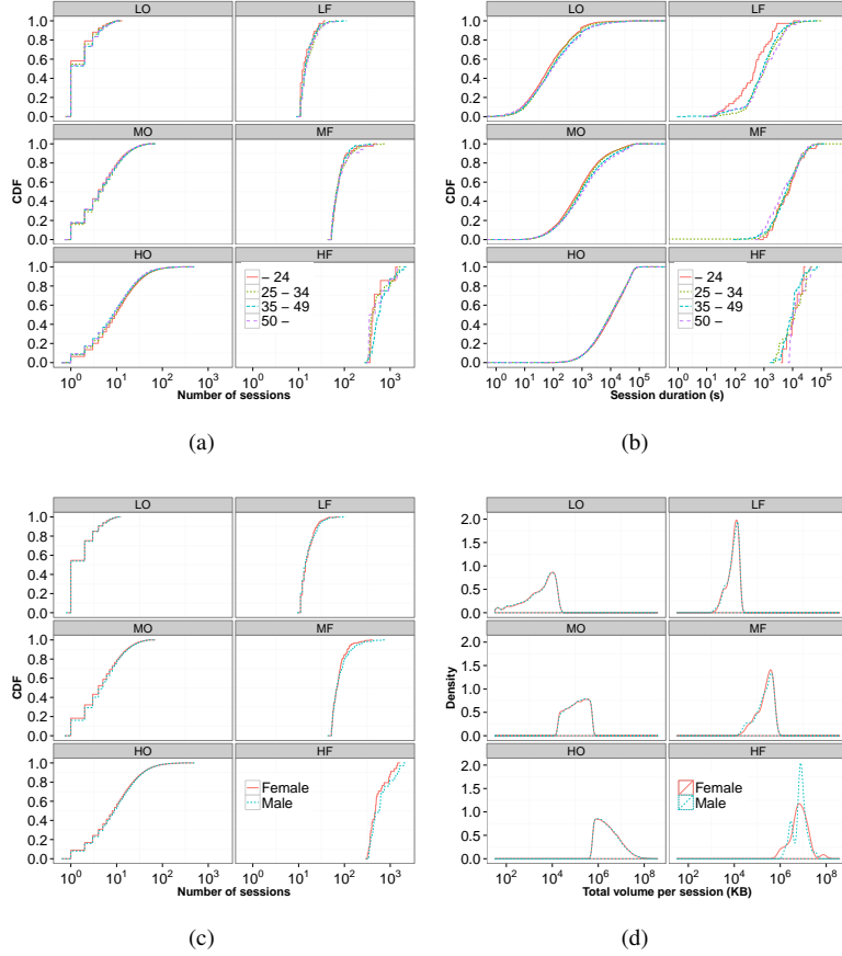
Figure 9: (a) CDFs of number of sessions and (b) session duration per subscribers' class and age range. (c) CDFs of number of sessions and (d) session volume per subscribers' class and gender.
