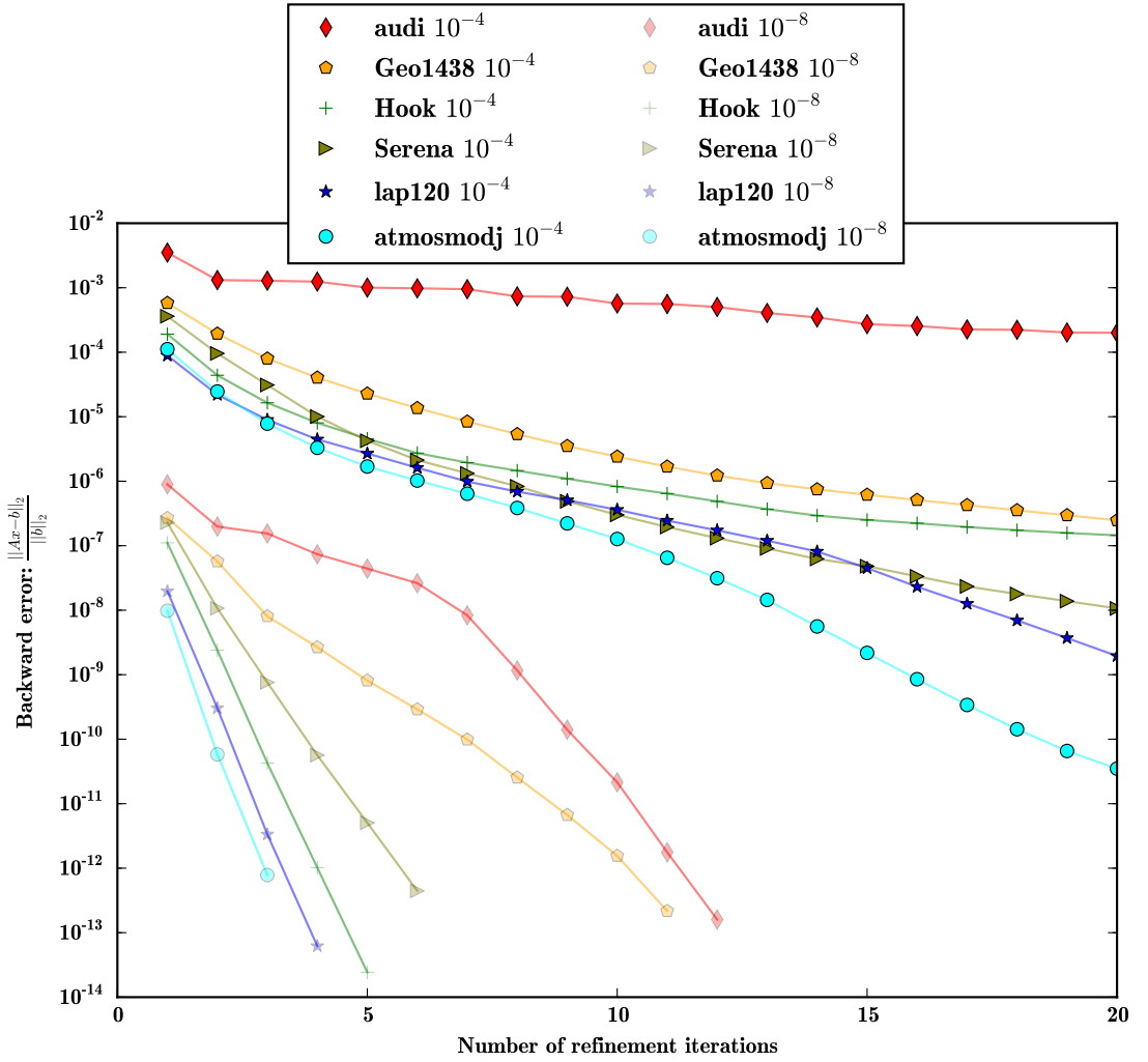
Figure 8: Convergence speed for the Minimal Memory /RRQR scenario with 2 tolerance thresholds.
