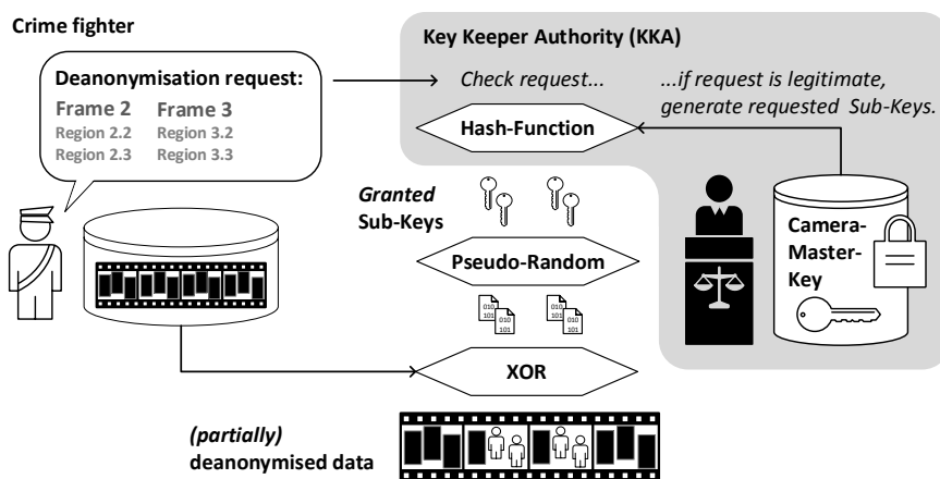
Fig. 2. De-anonymisation is only possible with the SKs granted by the KKA.
