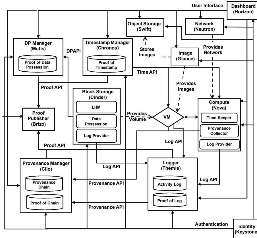
Figure 1. FECloud architecture.
