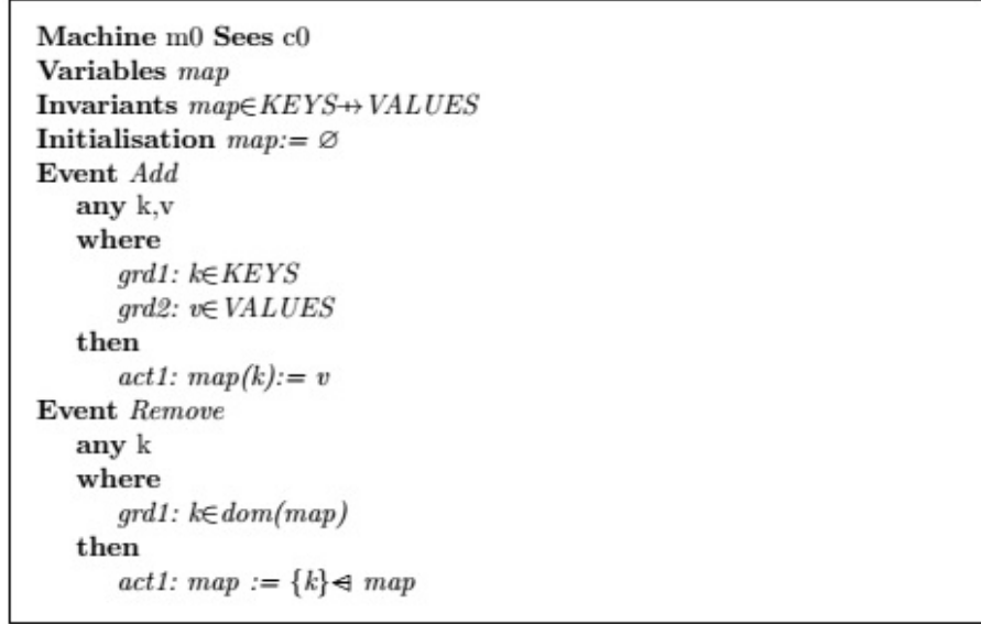
Fig. 1. Machine m0 : the Most Abstract Level of Map ADT Model
