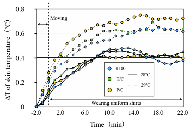
Fig. 9. Skin temperature
