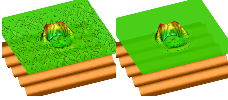
Figure 27: Moving steady states: evolution of a small perturbation in a homo-energetic steady state. 3D plot of the free surface. Left: approximation in physical variables. Right: approximation in steady invariants.
