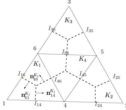
Figure 4: \mathbb{P}^2 residual distribution and finite volumes
