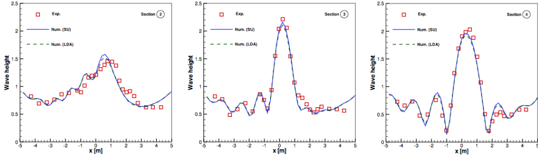
Figure 32: Wave scattering on an elliptic shoal. Time-average of the water height: simulations vs experiments.
