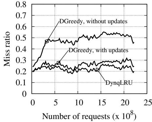
Figure 4: Impact of the popularity on DGREEDY policy: no updates in the estimate, with updated, and comparison with DYNQLRU.
