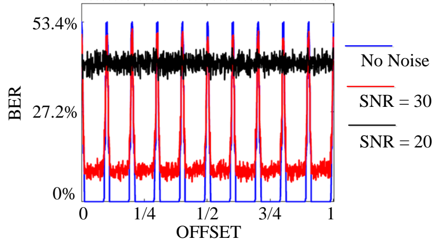
(b) Step with period equal to 10% of bit period
