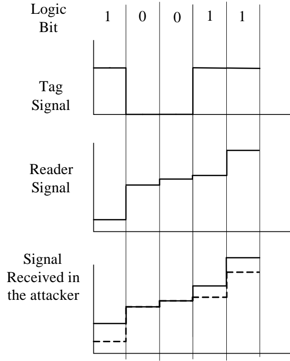
(a) Step period equal to bit period
