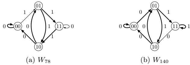
Fig. 6: De Bruijn graphs for W_{78} and W_{140}
