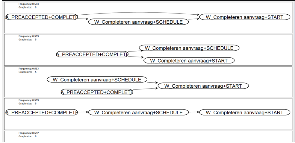
(a) View of discovered episodes (twelve in total)
