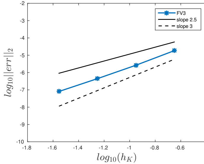
Figure 1: Grid convergence for the propagation of a 2D solitary wave
