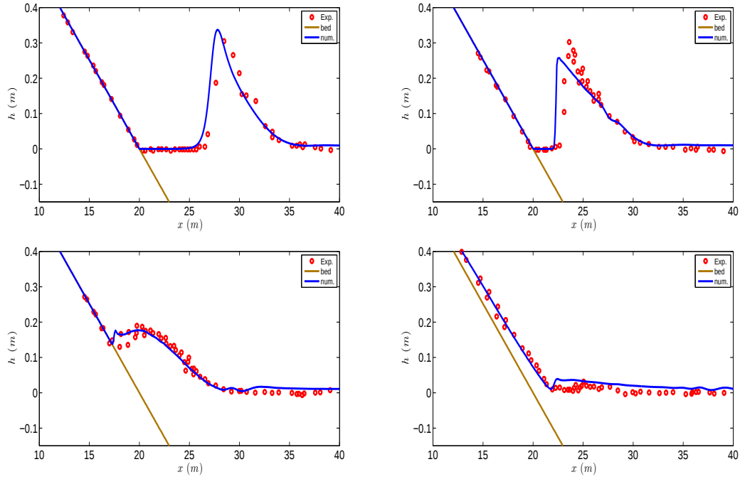
Figure 8: Solitary wave run-up on a plane beach: snapshots of the free surface elevation for dimensionless times t\sqrt{g/h} = 15, 20, 25, 45 (from left to right and top to bottom ).
