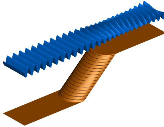
Figure 2: Shoaling of regular waves, case (a): perspective view of the free surface
