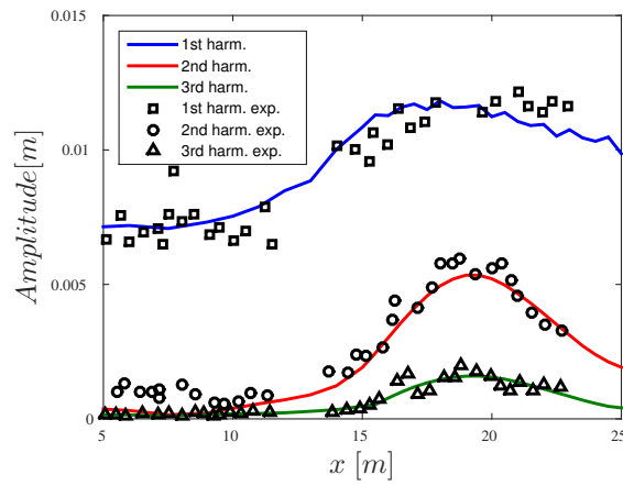
Figure 7: Shoaling of regular waves, case(b): comparison of the computed and experimental results for the wave amplitudes for the first and second harmonics along the centreline
