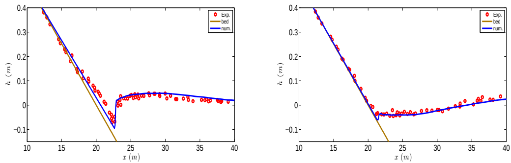
Figure 9: Solitary wave run-up on a plane beach: snapshots of the free surface elevation for dimensionless times t\sqrt{g/h} = 60, 80 .
