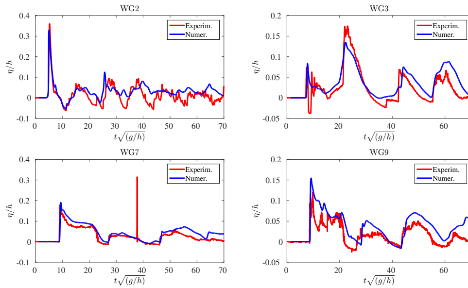
Figure 12: Solitary wave propagation over a three dimensional reef: computed time series of the free surface elevation on gauges positions
