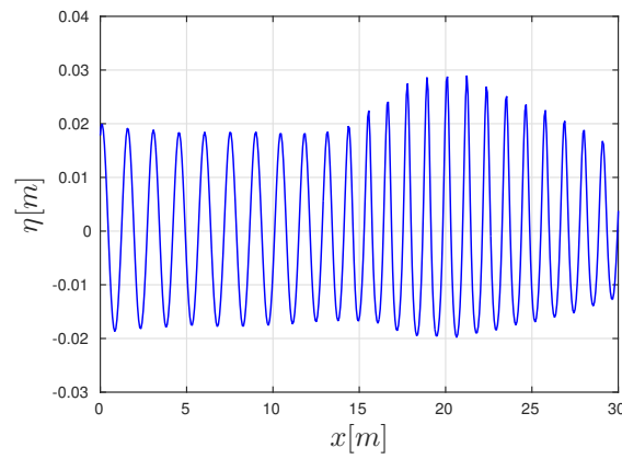
Figure 3: Shoaling of regular waves, case(a): surface elevation along the centreline
