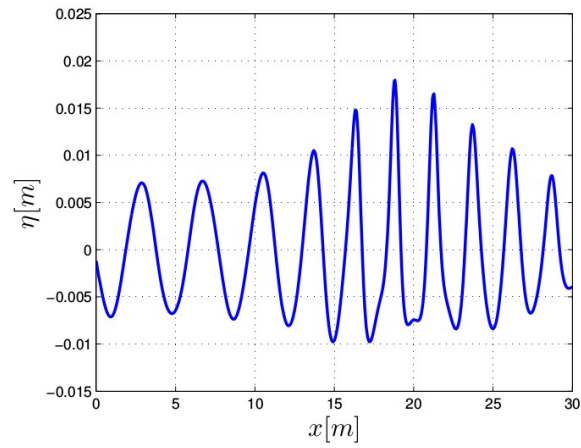
Figure 6: Shoaling of regular waves, case(b): surface elevation along the centreline
