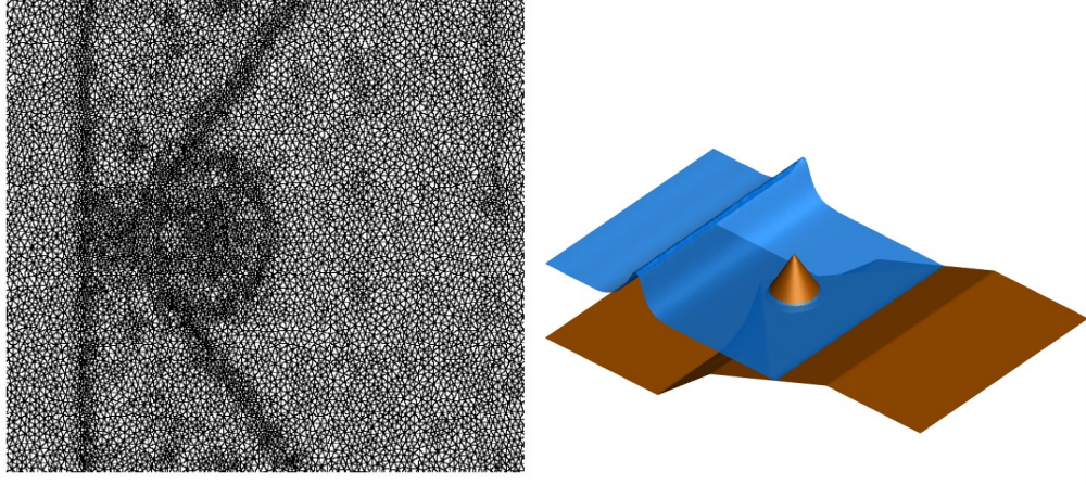
Figure 10: Solitary wave propagation over a three dimensional reef: Close up view of the adapted mesh used for the computation(left) and computed free surface solution with friction at times t = 3.5s .
