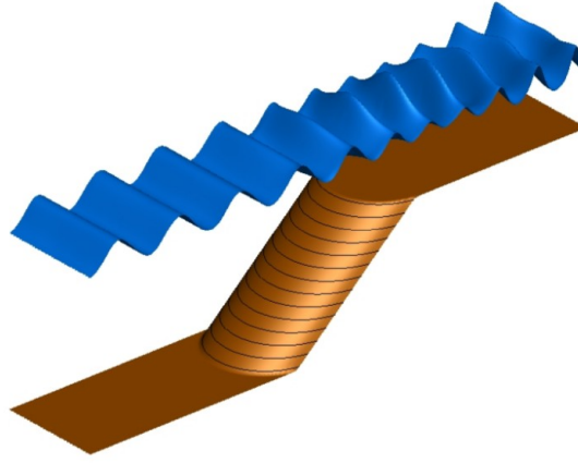
Figure 5: Shoaling of regular waves, case (b): perspective view of the free surface
