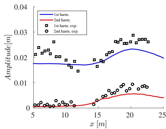
Figure 4: Shoaling of regular waves, case(a): comparison of the computed and experimental results for the wave amplitudes for the first and second harmonics along the centreline
