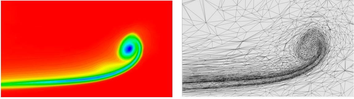
Figure 16: M6 wing example: Wing tip vortex 8 body-length behind the wing.
