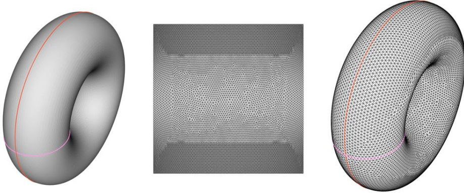
Figure 4: From left to right, CAD of a torus with 2 edges and one face, 2D mesh in the parametric space, and mapped uniform surface mesh.
