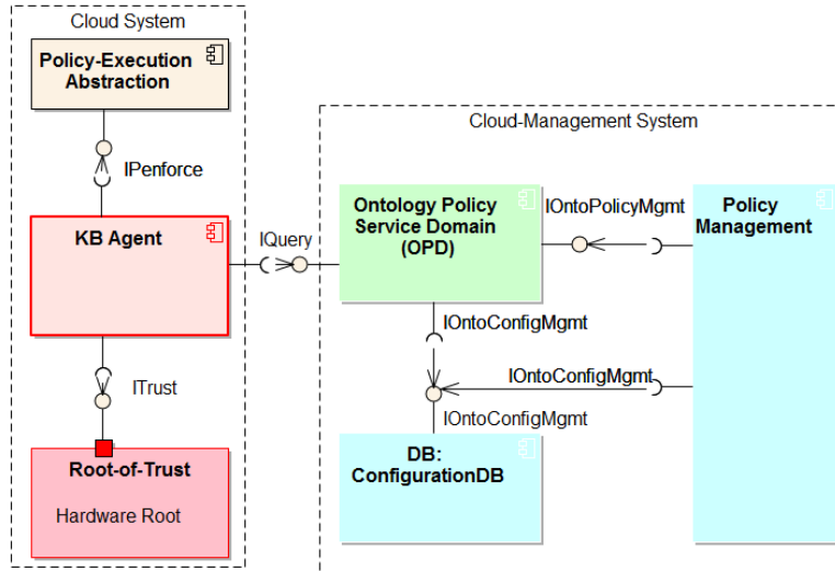
Fig. 1. Knowledge-based agent architecture
